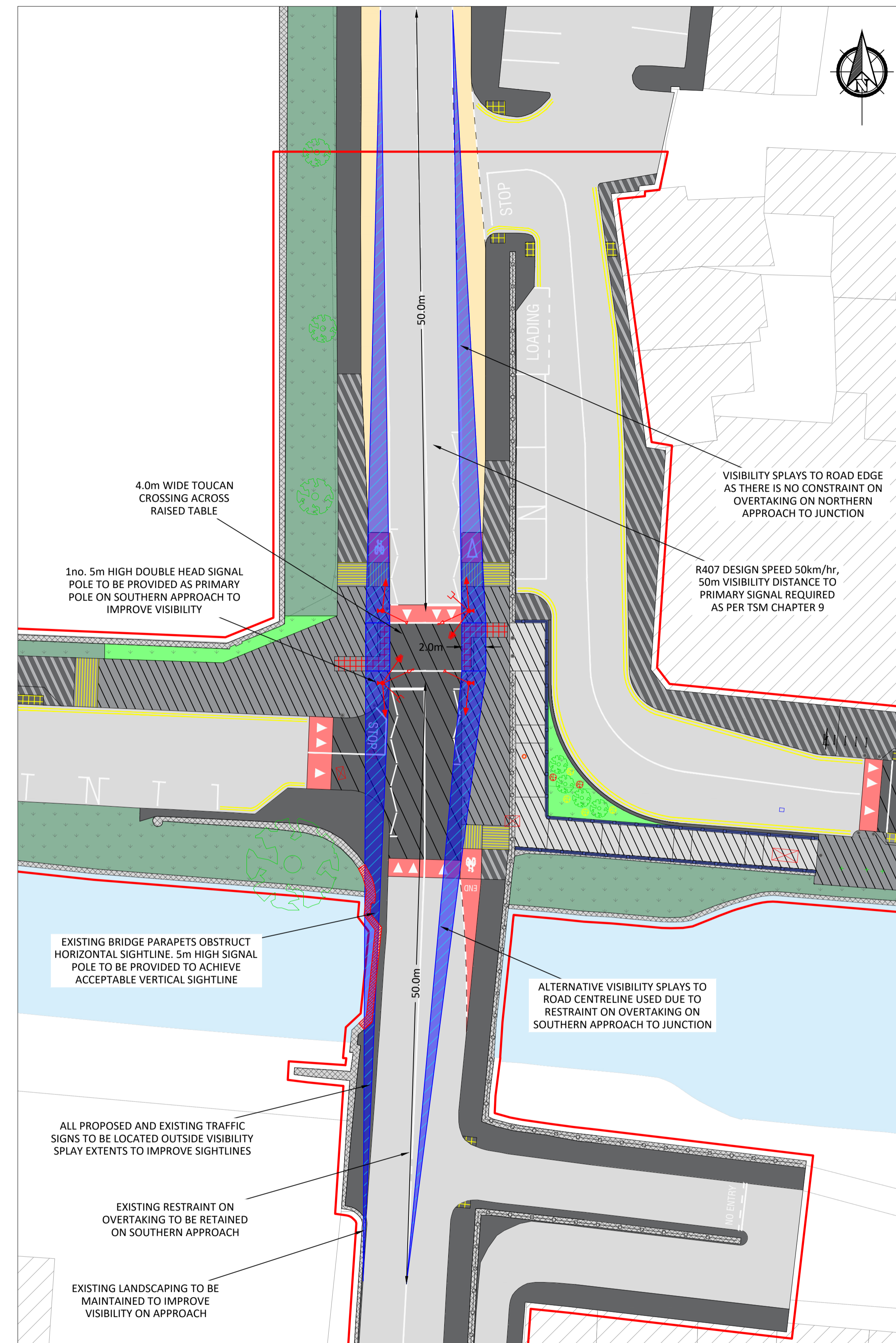
TOUCAN CROSSING - HORIZONTAL SIGHTLINES Scale 1:250
