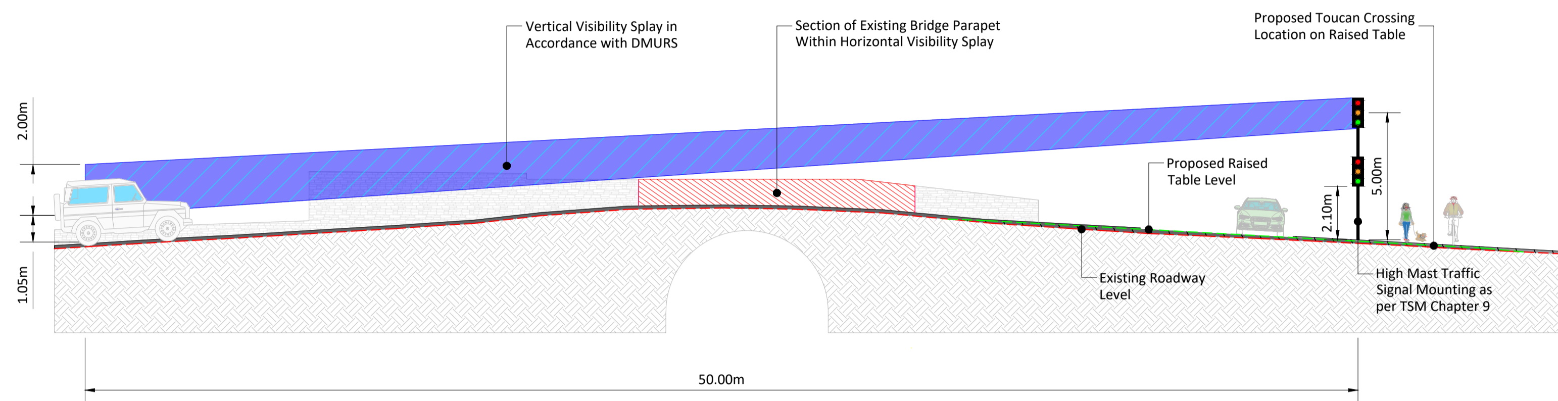
TOUCAN CROSSING - VERTICAL SIGHTLINES Scale 1:150
